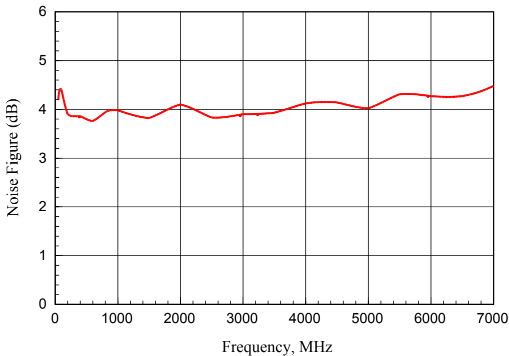
ABL0600-01-3440 Measured Noise Figure vs Frequency
