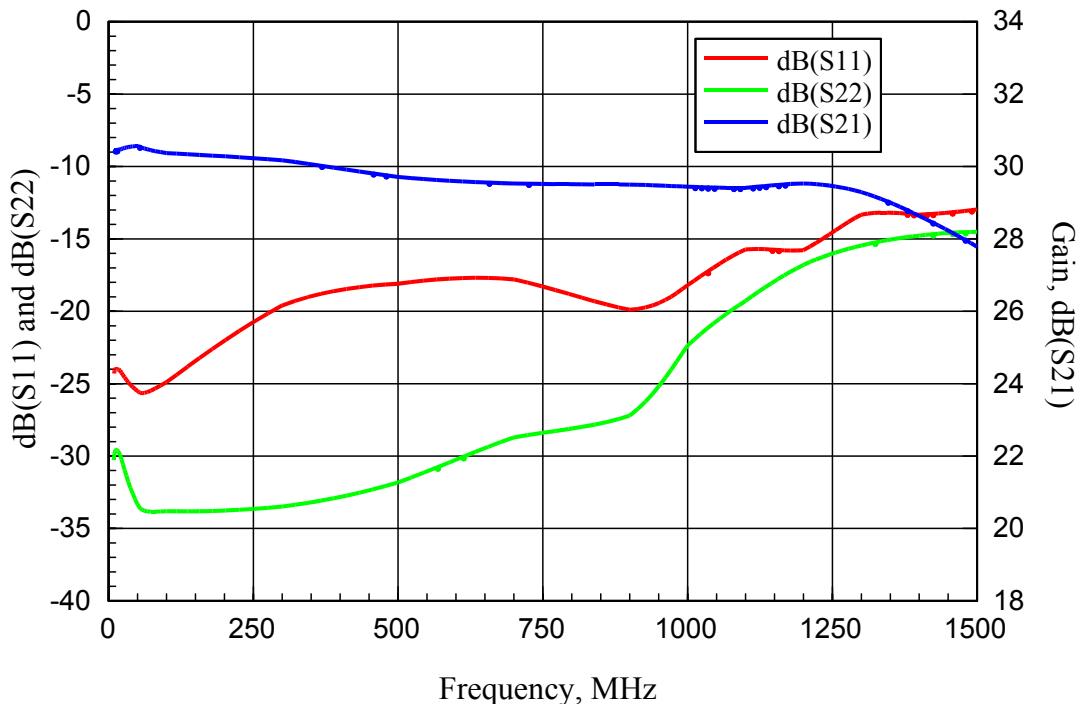
ABL0100-01-3010 Measured Gain and Return Loss vs Frequency
